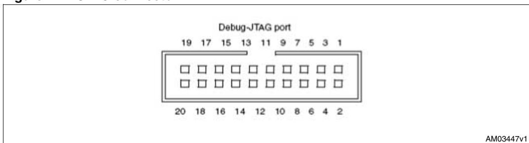
Figure 11. JTAG connector
