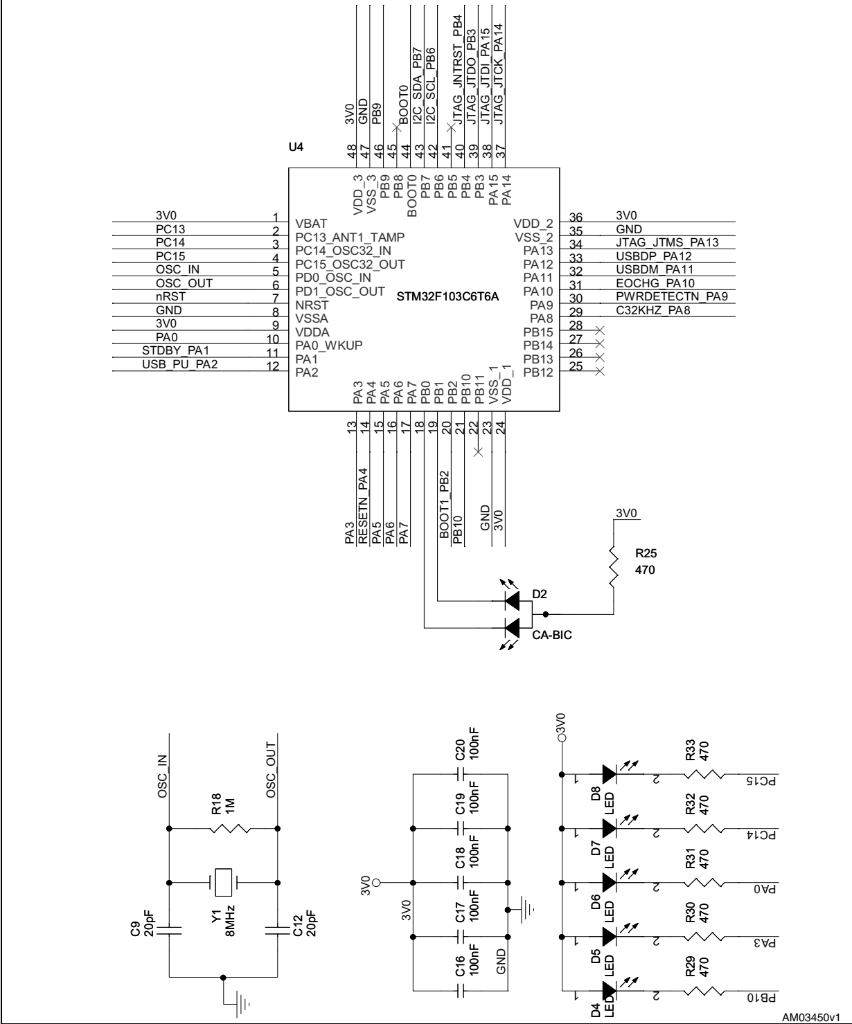
Figure 14. Microcontroller section schematic
